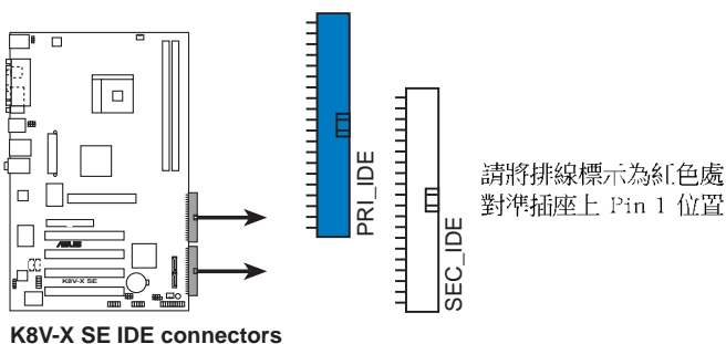
K8V-X SE IDE connectors
