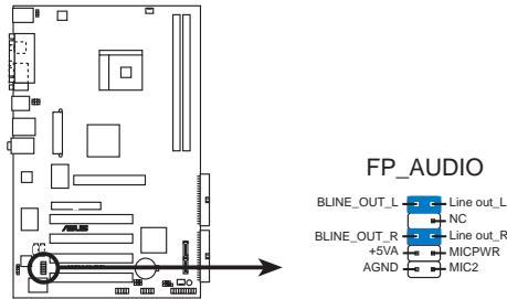
K8V-X SE Front panel audio connector
