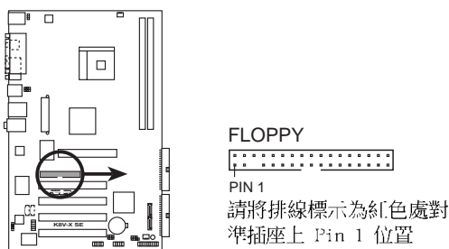
K8V-X SE Floppy disk drive connector
