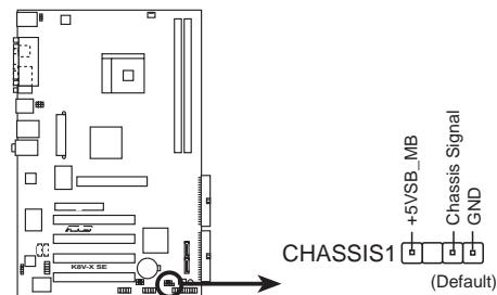
K8V-X SE Chassis intrusion connector
