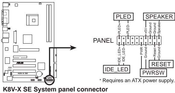
K8V-X SE System panel connector
